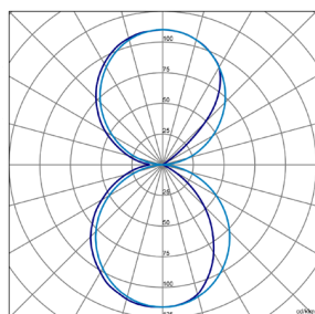
ECOSTAIR-1690-78W
